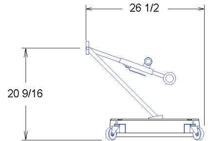
SIDE VIEW WITH HANDLE FOLDED
